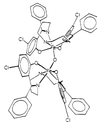
Figure 1. Scale drawing of the [Fe(cbpN)] 2 O molecule.
